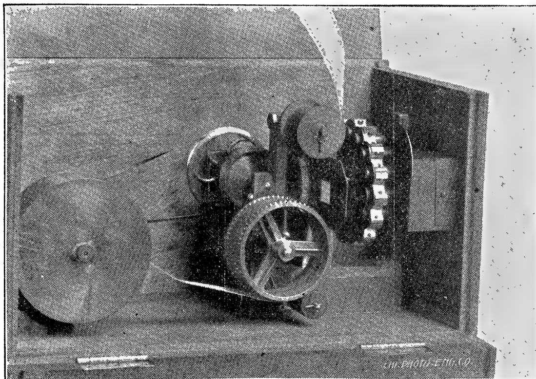
JENKINS' ROTARY LENS CAMERA.
